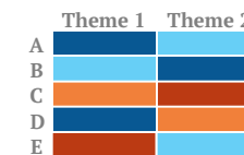
Heat Map
