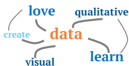
Phrase Net
