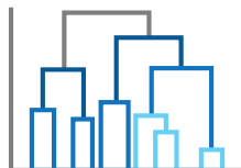
Dendrogram
